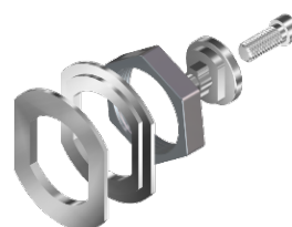
AG50.4 Swedish tail piece set for Swedish type of cams
